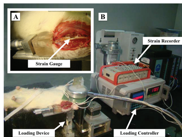
Figure 1. Setup of the axial tibial loading scenario and the in vivo rat tibia strain recording. A: A strain gauge was attached on the tibia surface. B: In vivo strain was recorded under mechanical loading.
