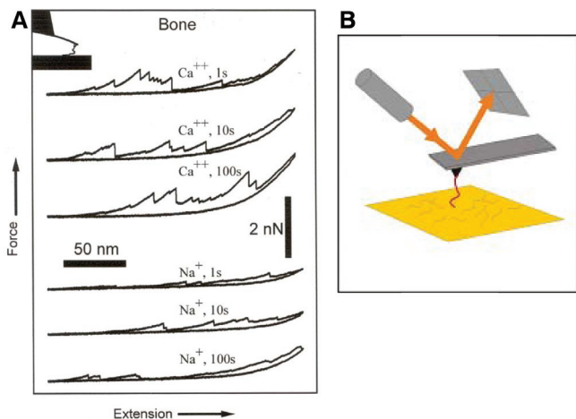
Figure 1. A. Atomic Force Microscope (AFM) force vs extension curves of pulled bone molecules demonstrate that the sacrificial bonds of polymers of the organic matrix of bone are much harder to rupture in the presence of Ca^{++} ion than an Na^+ buffer. (Thompson et al. Nature 2001; 414:773-776). B. AFM molecular pulling: a cantilever stretching a molecule deflects according to the molecule's properties; a laser beam focused on the cantilever and reflected to a diode records the cantilever's deflections.
