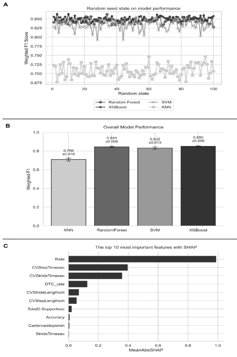
Figure 2. (A) Effect of random seed state on model performance across 100 repetitions. (B) Overall model performance comparison among k-nearest neighbor (KNN), random forest, support vector machine (SVM) and extreme gradient boosting (XGBoost). Each Weighted F1 score was averaged across 100 repetitions with incrementing random seed. Error bar indicates standard deviation between 100 random states. (C) The top ten most important features, ranked by their mean absolute SHAP values (MeanAbsSHAP) for XGBoost classifier. The features are shown from top to bottom in order of importance. Note: SHAP – SHapley Additive exPlanations; Rate – Rate of response (characters/sec); CVStepTimesec – Coefficient of variation (%CV) of step time; CVStrideTimesec – Coefficient of variation (%CV) of stride time; DTC_rate – Dual task cost of rate; CVStrideLengthcm – Coefficient of variation (%CV) of stride length; CVStepLengthcm – Coefficient of variation (%CV) of step length; TotalD.Supportsec – total double support time; Accuracy – Response accuracy (number of correct responses/total number of answers provided); Cadencestepsmin – cadence (steps/minute); StrideTimesec – stride time.
